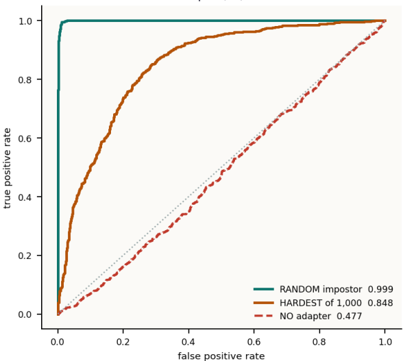
Experiment B · MobileCLIP-S1 → SigLIP 2 0.79 MB adapter, 1,000 held-out
